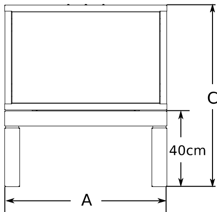
ΠΡΟΟΨΗ FRONT VIEW
